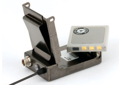
Power is provided by a rechargeable lithium-ion battery
